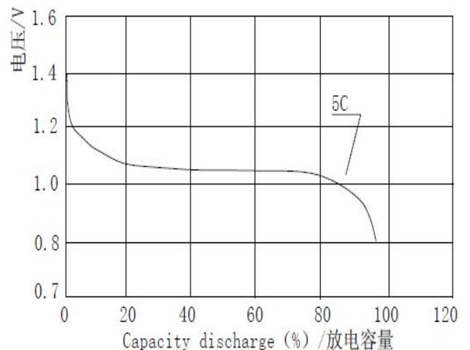
High rate discharge/高倍率放电
