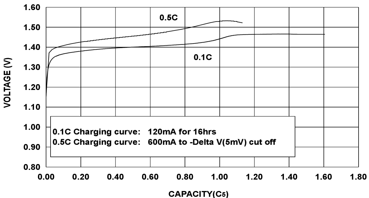
CHARGING CURVE OF BPI-50AA1200 CELL
