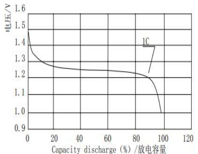
High rate discharge/高倍率放电
